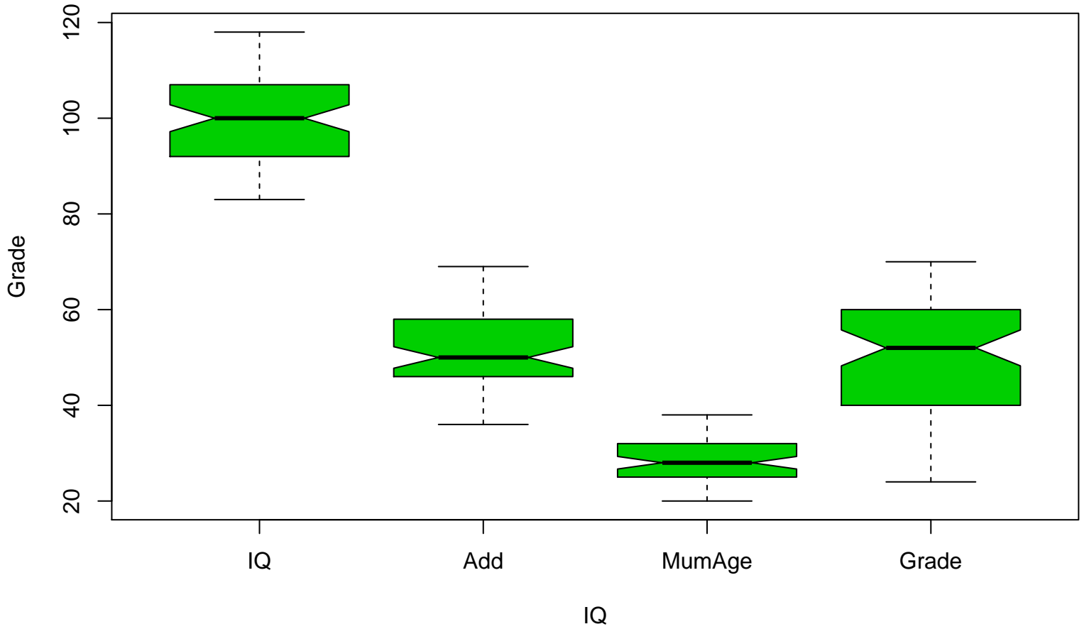
IQ and Grade regression – 10% trim
