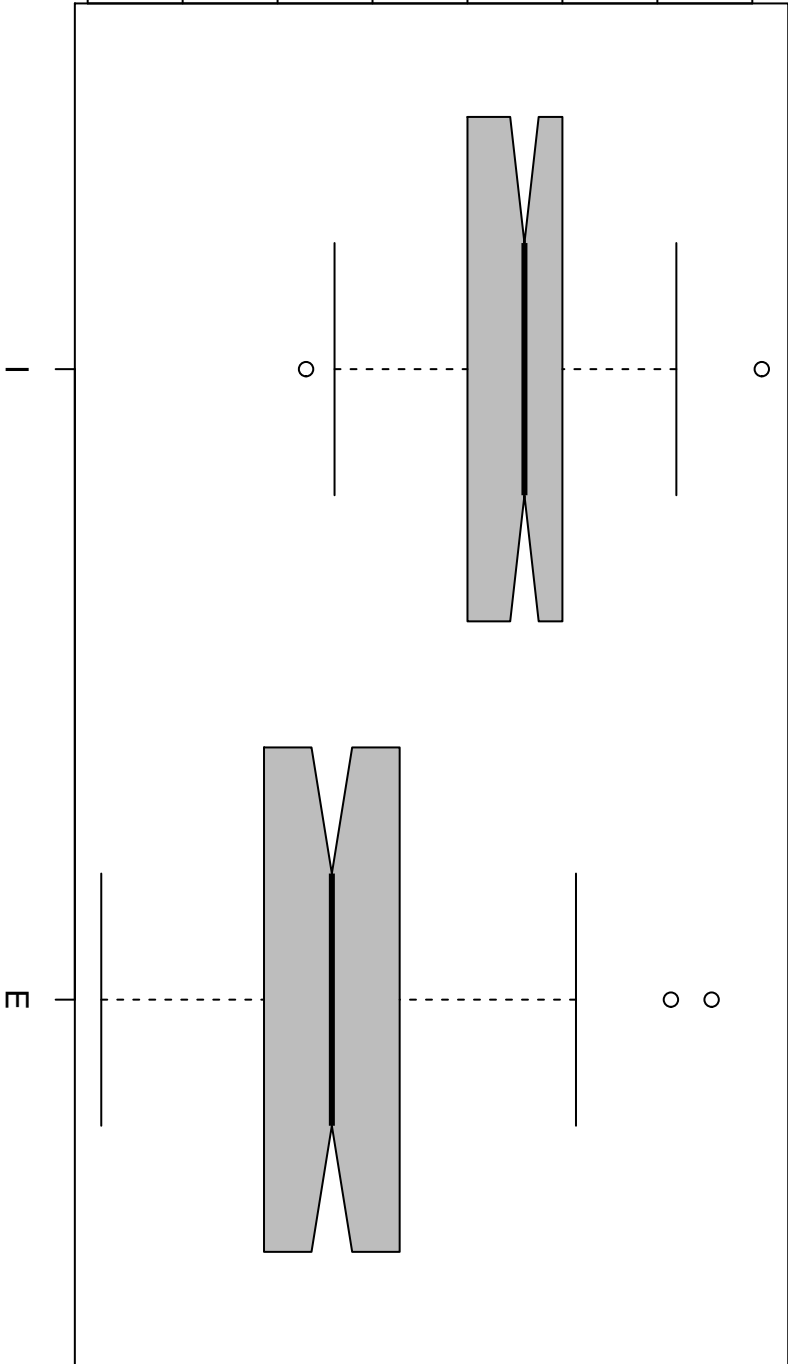
Notched Boxplots
