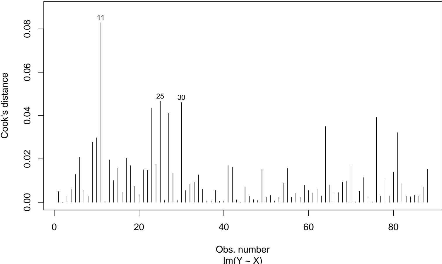
Cook's distance
