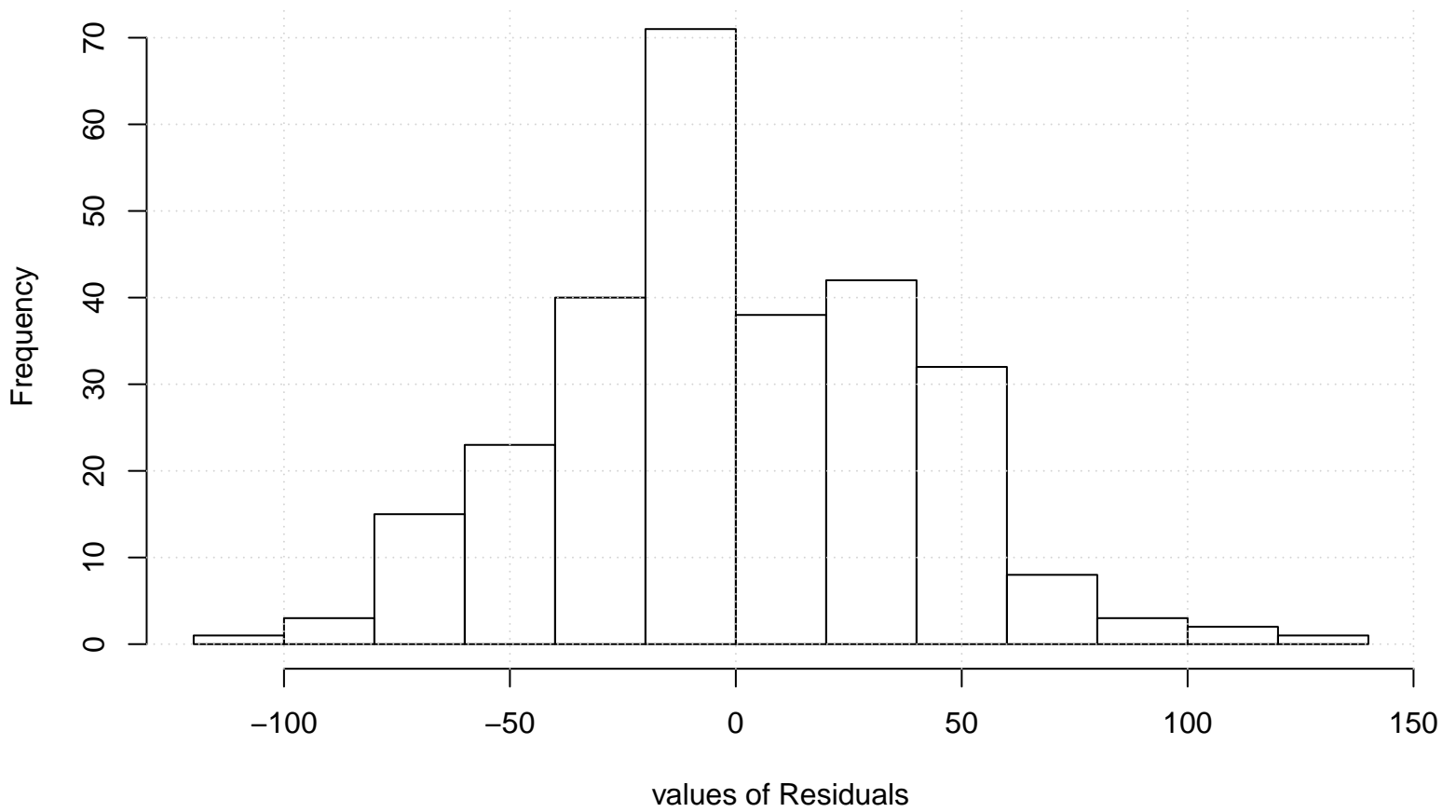
Residual Histogram
