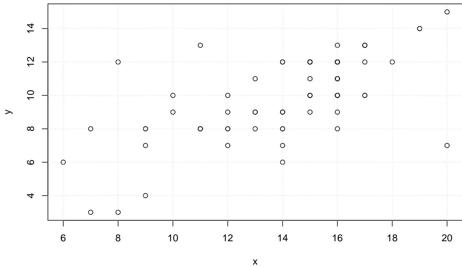
Scatterplot
