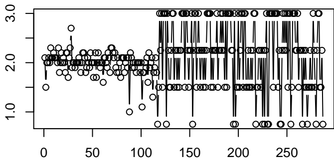
Plot of x
