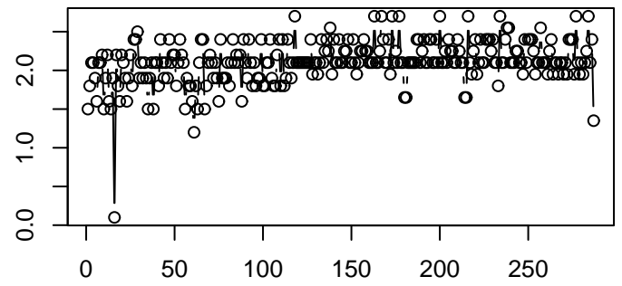
Plot of y
