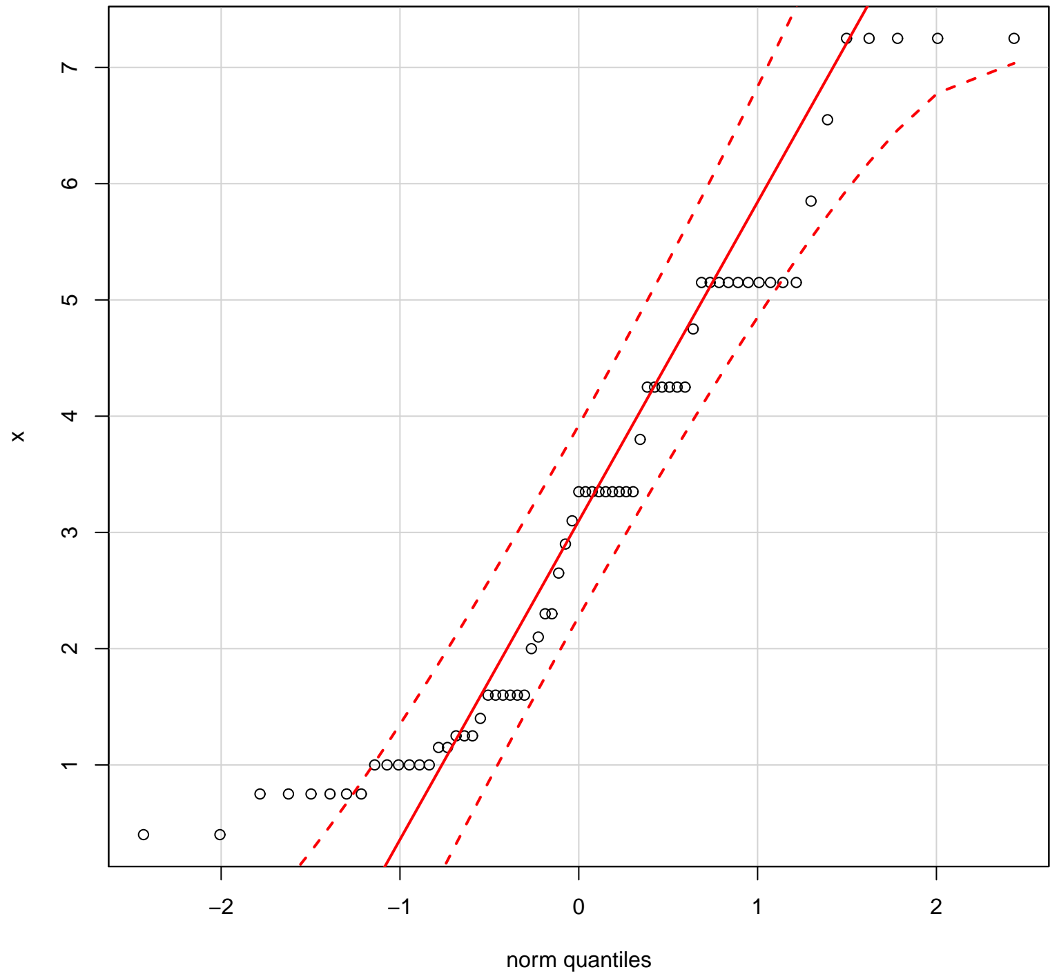
QQplot of variable x
