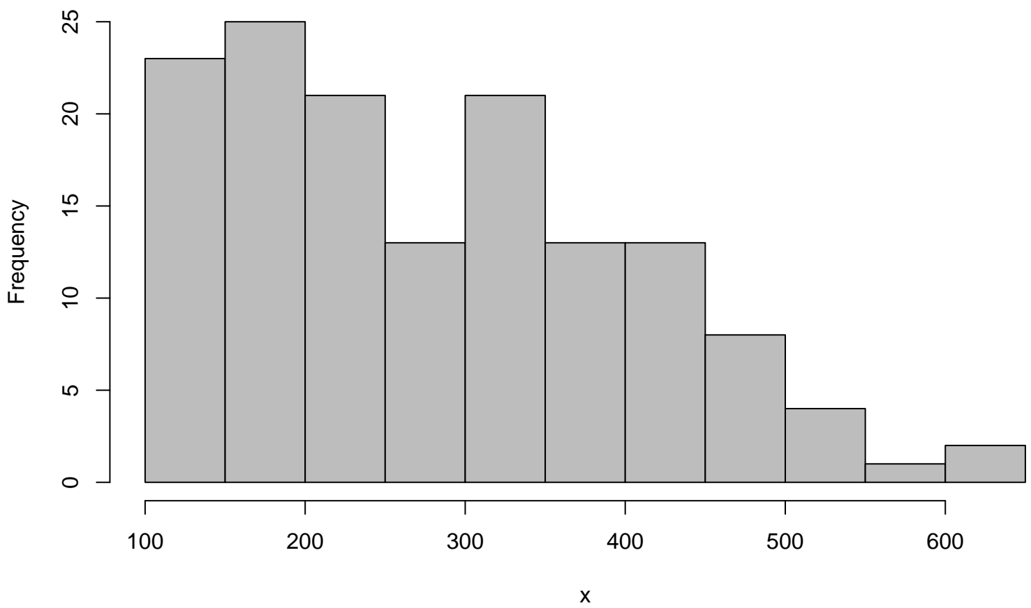
Histogram Numercy Score
