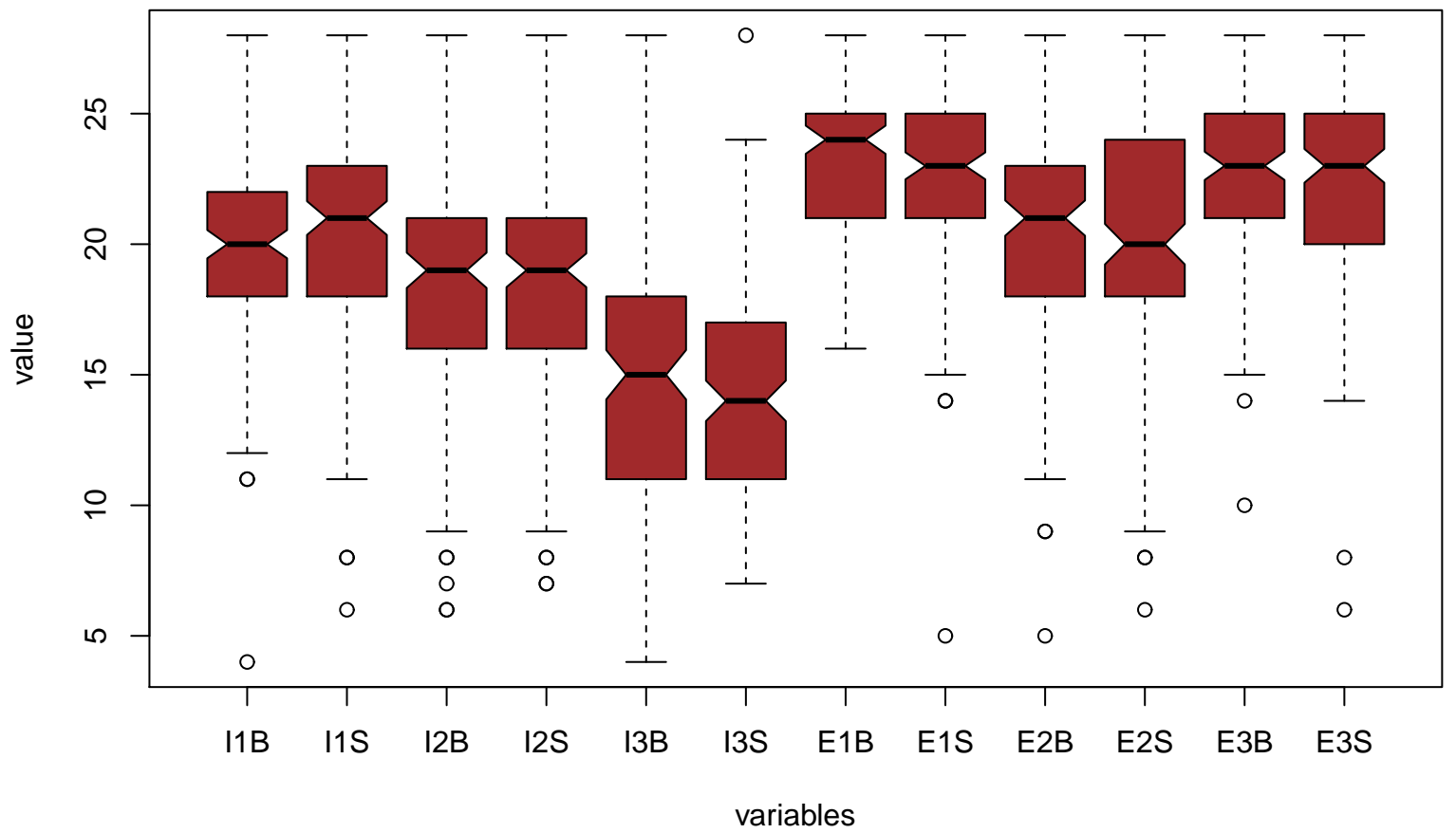
Notched Boxplots
