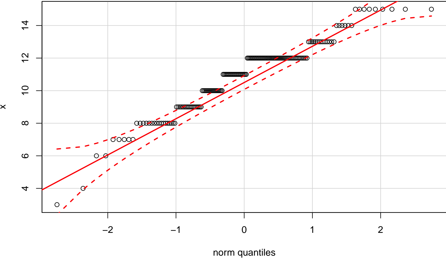
QQplot of variable x
