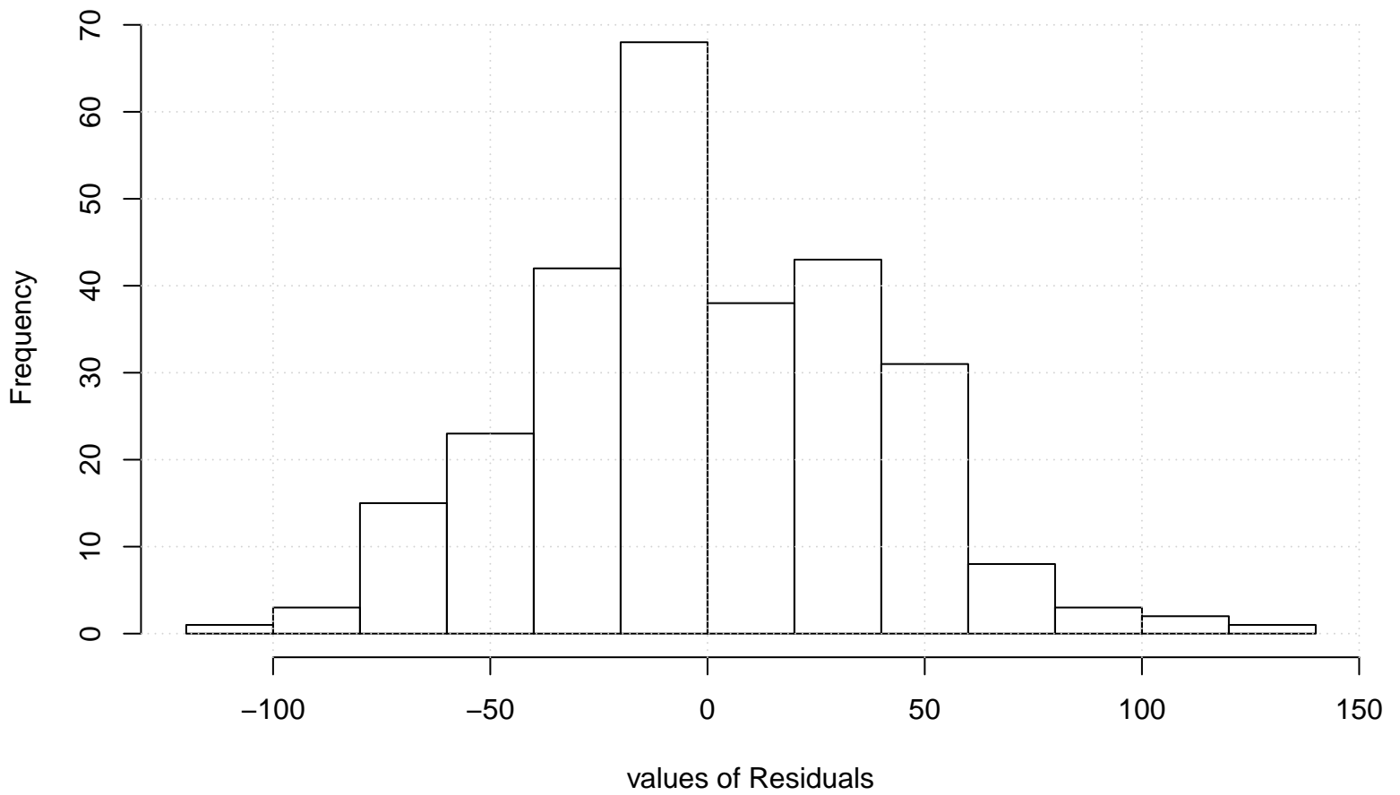
Residual Histogram
