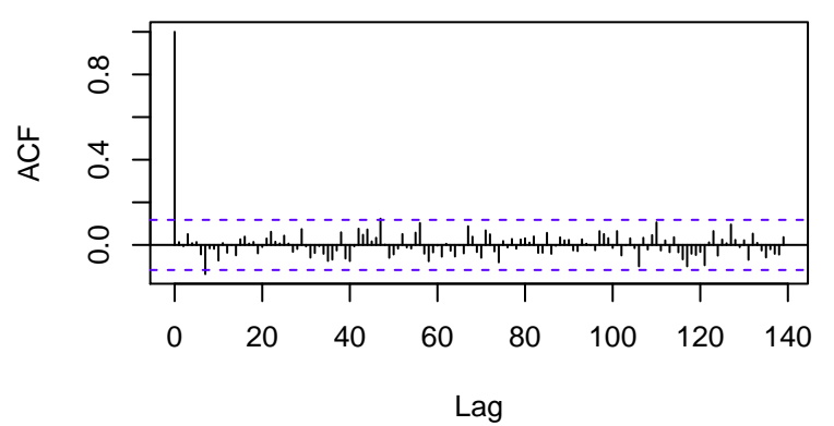
Standardized Residuals
