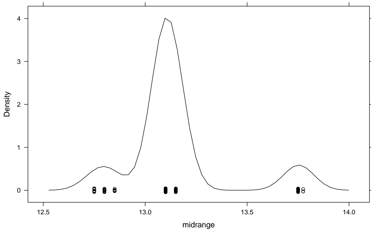
Density Plot
