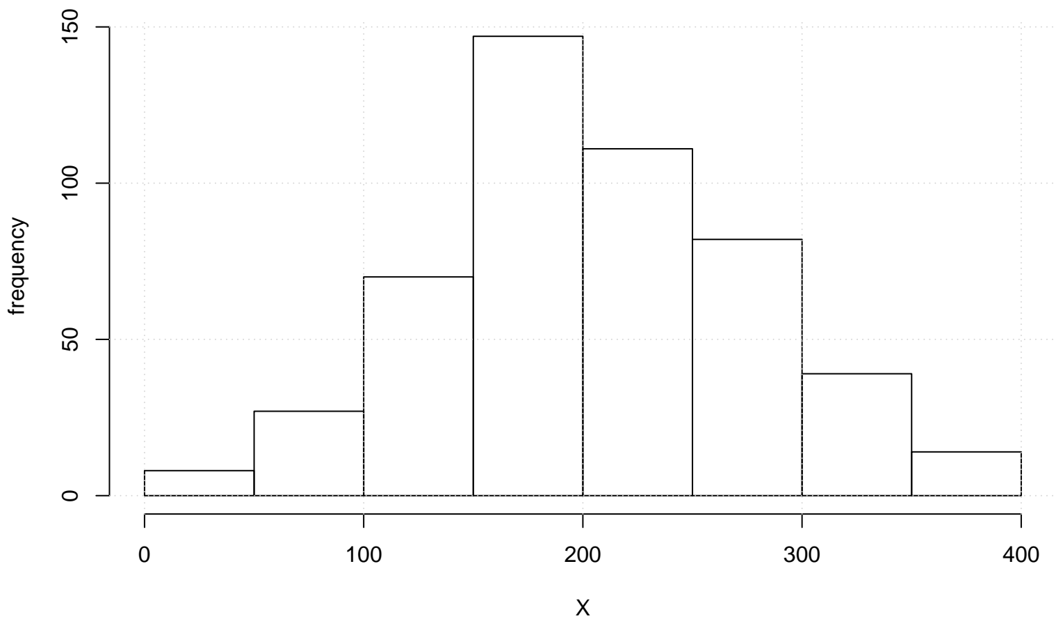
Histogram of Transformed Data
