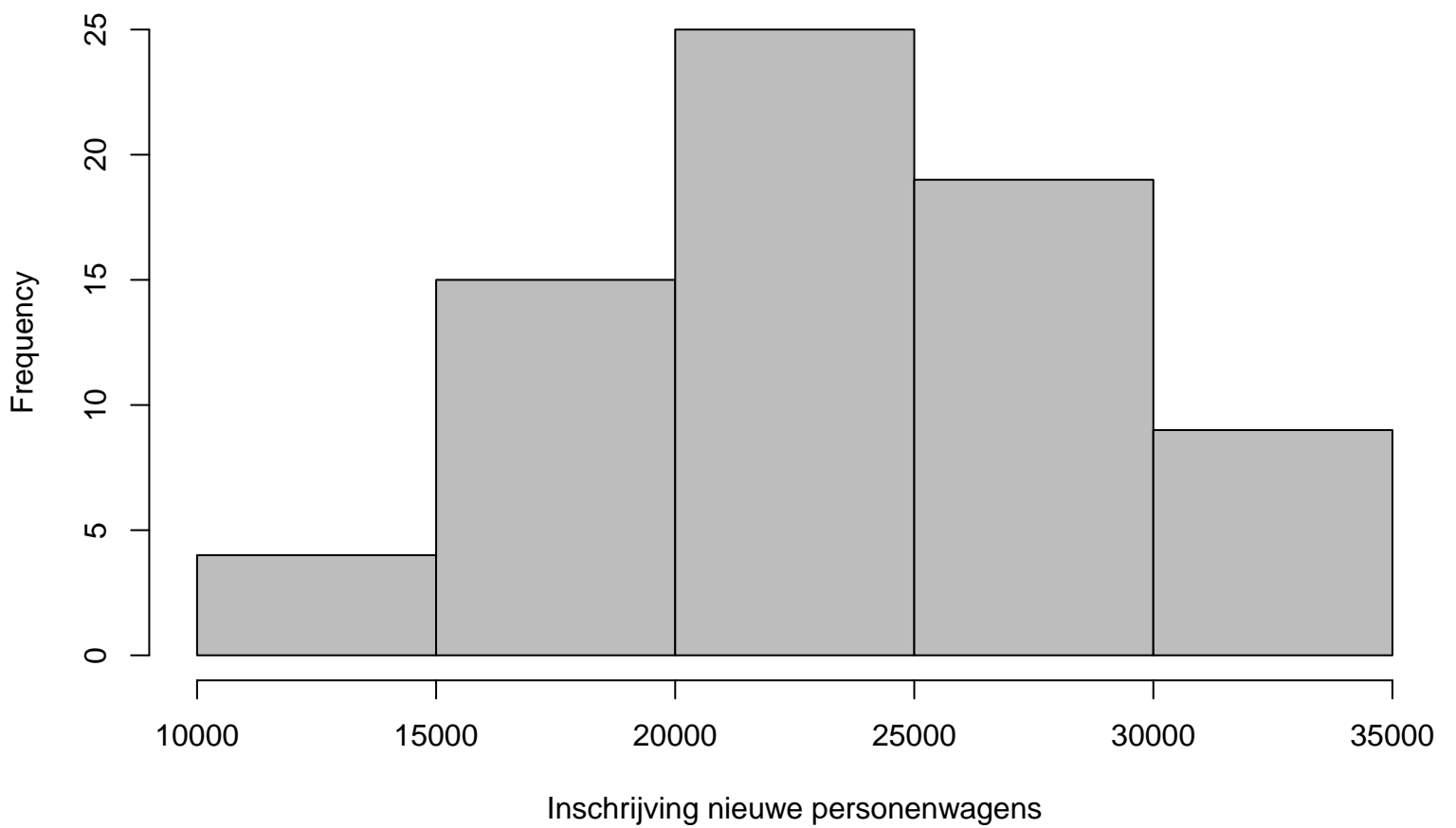
Histogram
