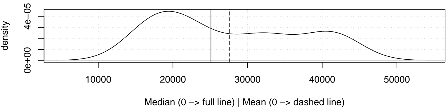
Density Plot – Gaussian Kernel
