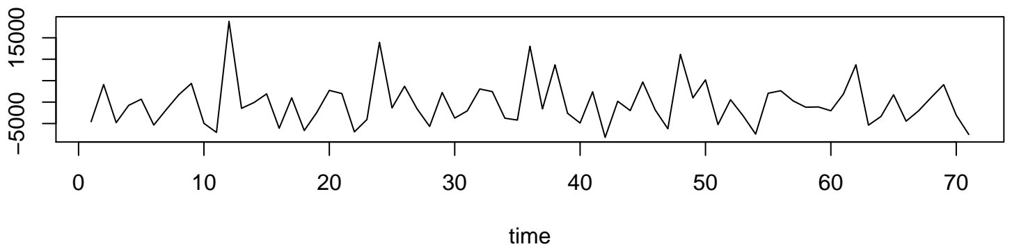
Working Time Series ( \lambda=1 , d=1 , D=0 )
