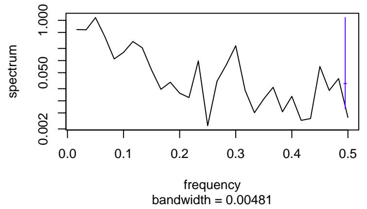
Random
