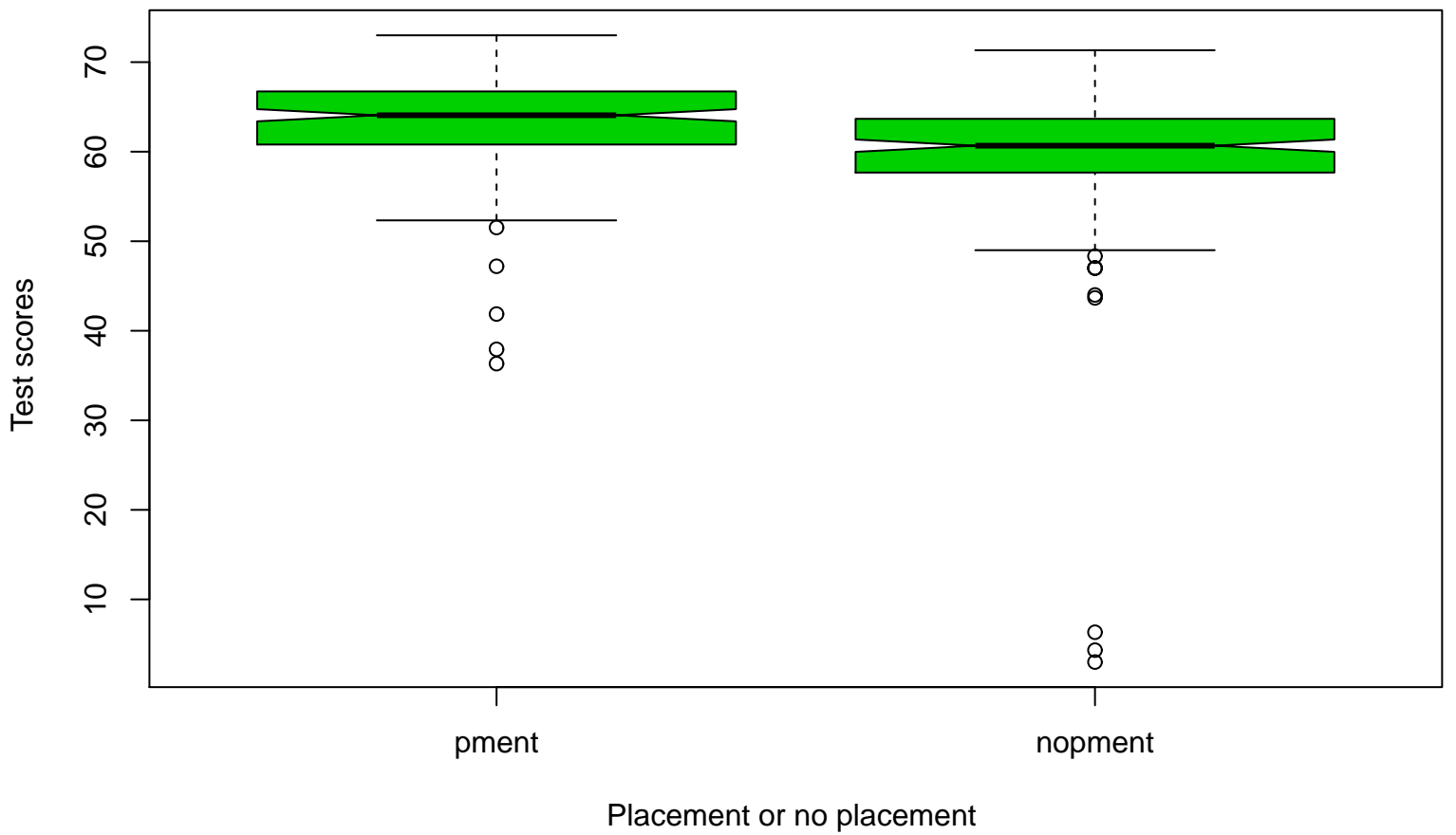
placement vs no placement scores
