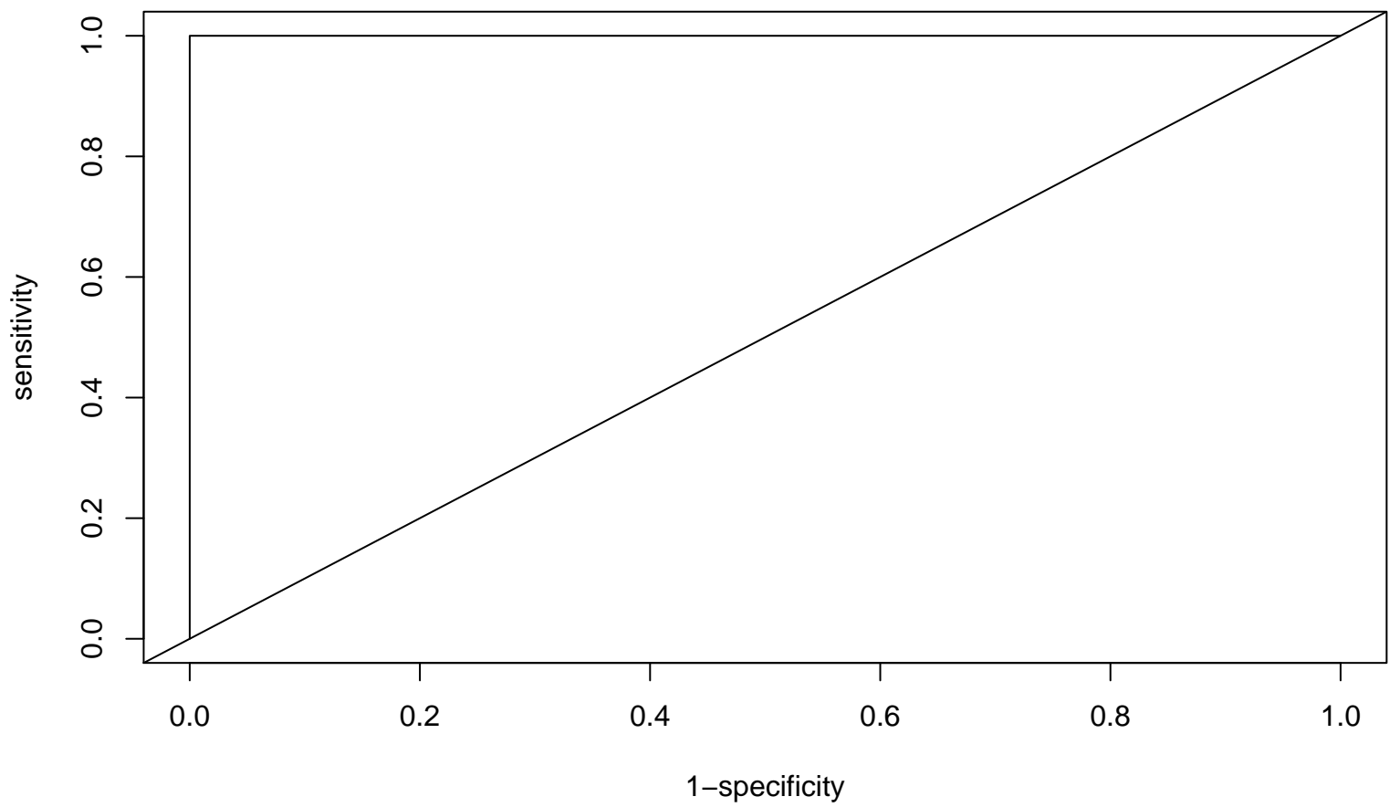
ROC plot
