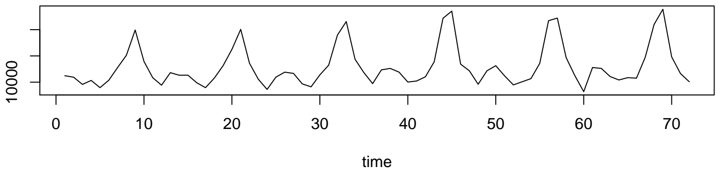
Working Time Series ( \lambda=1, d=0, D=0 )
