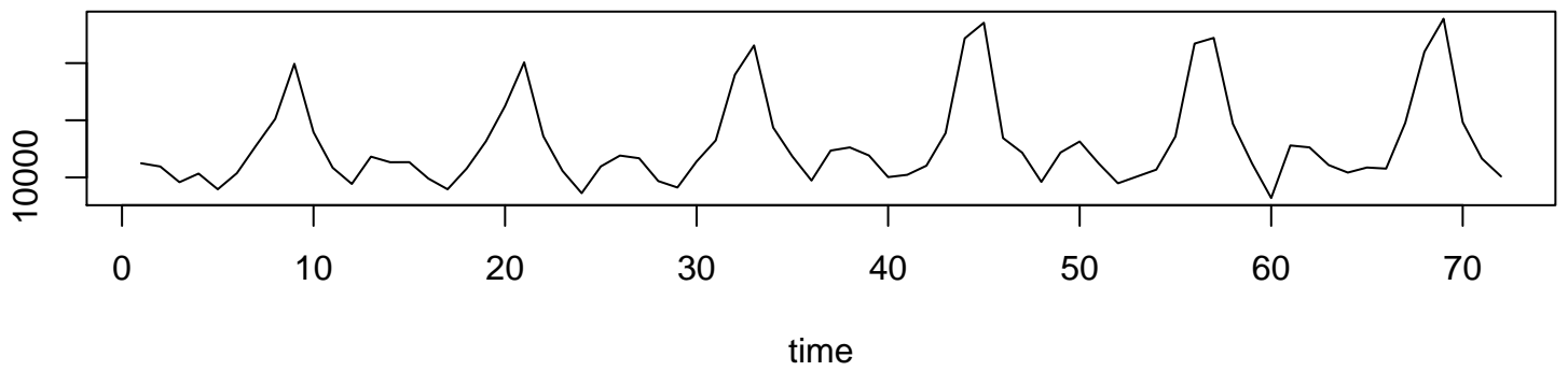
Original Time Series
