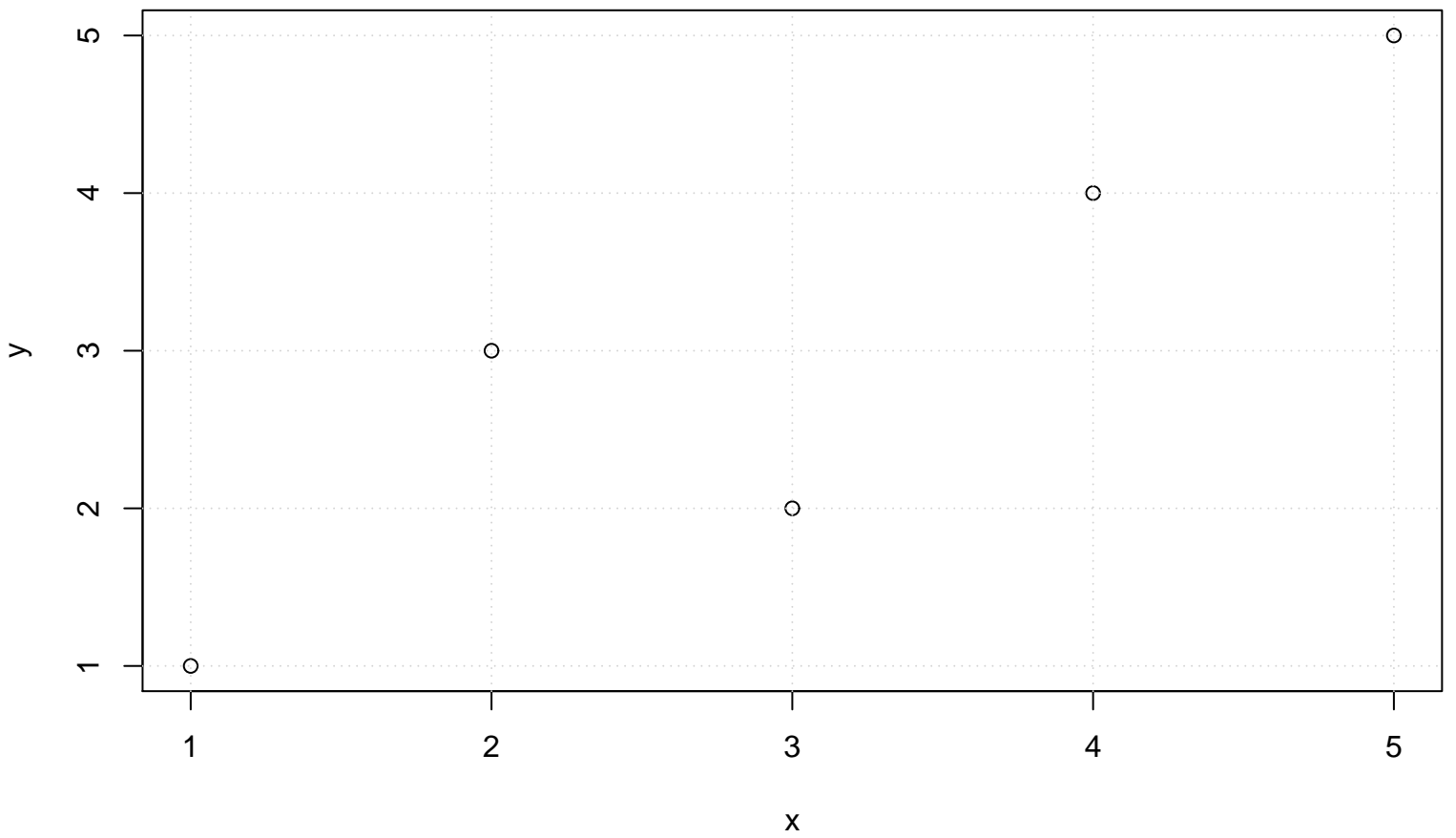
Scatterplot of Ranks
