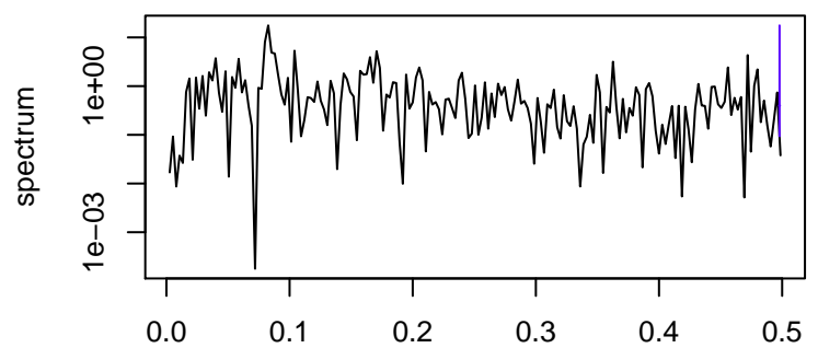
Standardized Residuals
