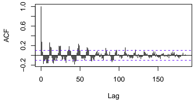
Standardized Residuals
