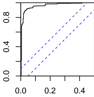
Observed
