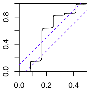
Seasonal
