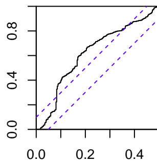
Standardized Residuals
