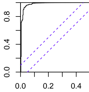
Level
