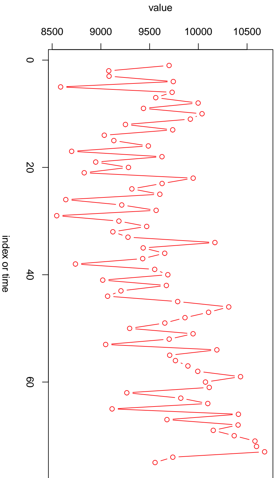
Univariate Data
