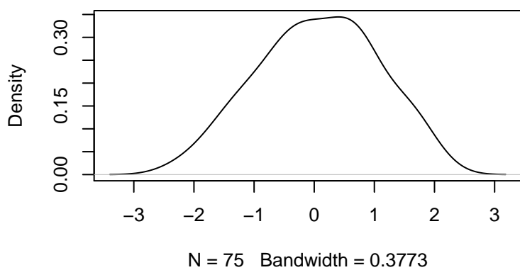
Residual Kernel Density
