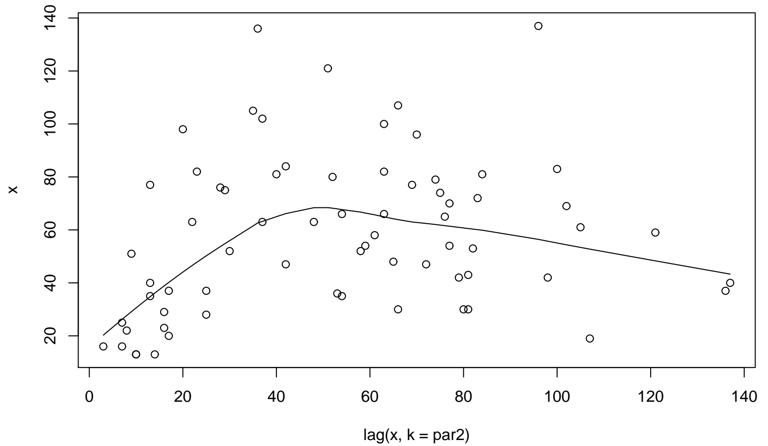
Lag plot (k=11), and lowess
