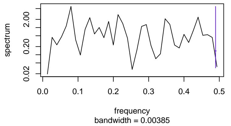
Standardized Residuals
