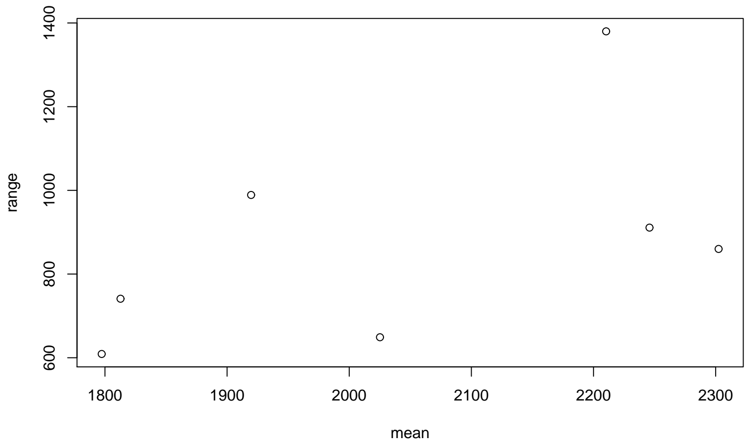
Range-Mean Plot
