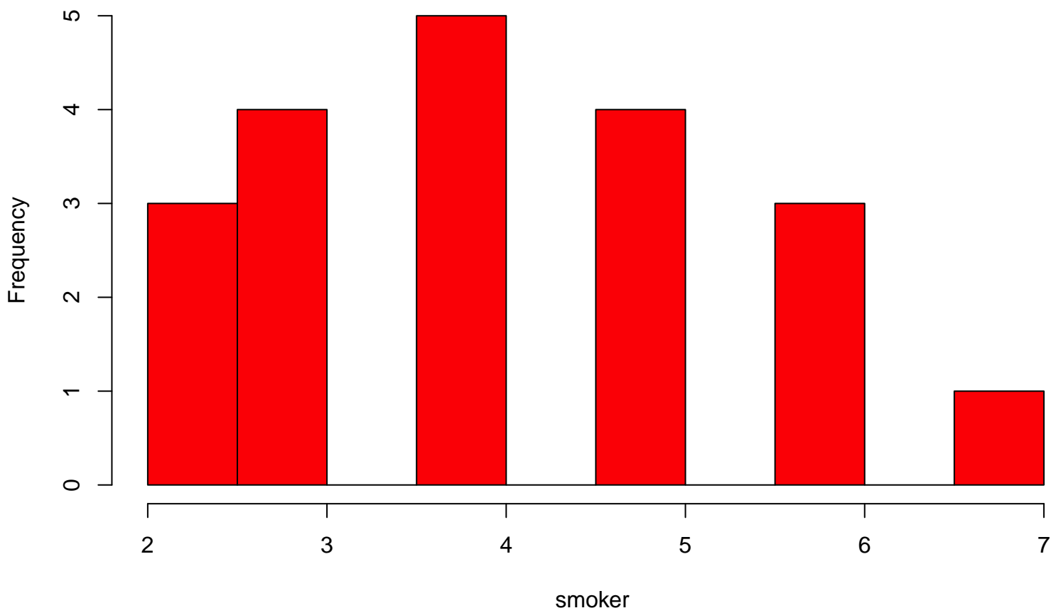
Histogram for SMK and hot curry
