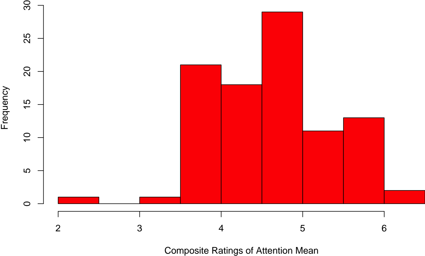
Distribution of compattenmean
