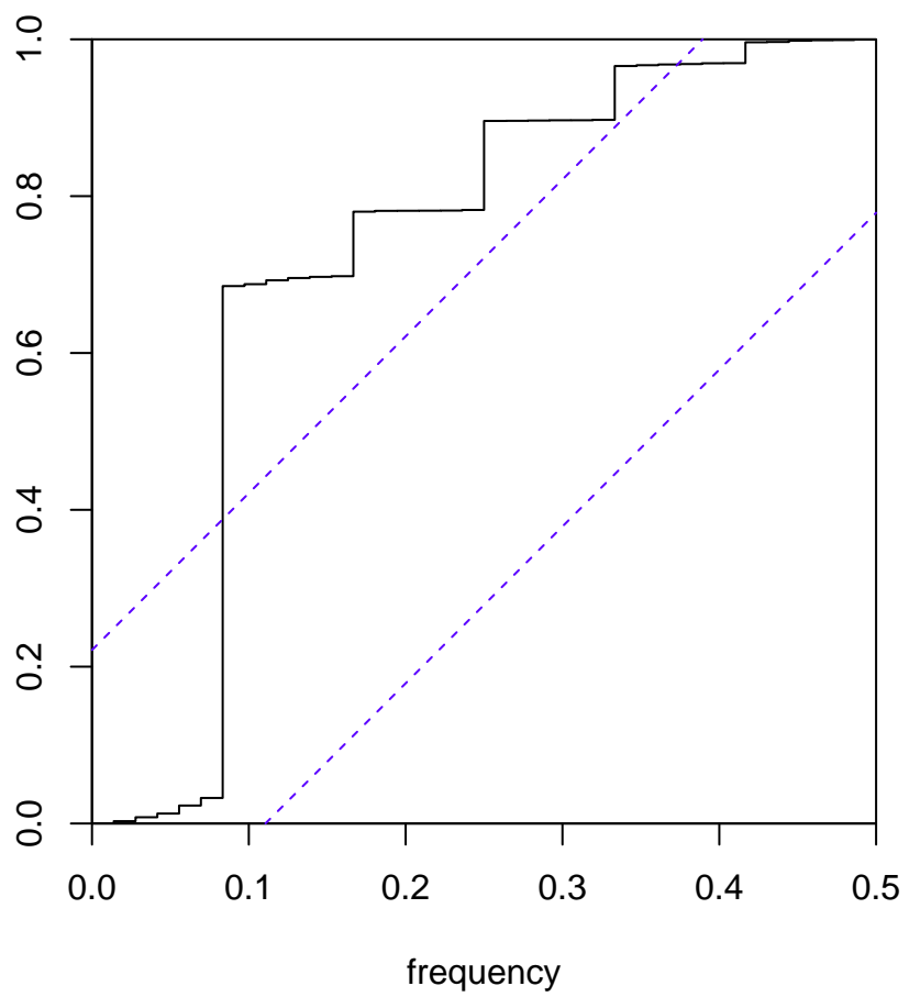
Cumulative Periodogram
