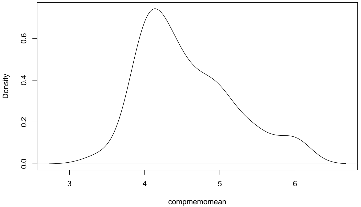
compmemomean QQplot
