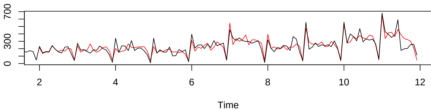
Interpolation Fit of Exponential Smoothing
