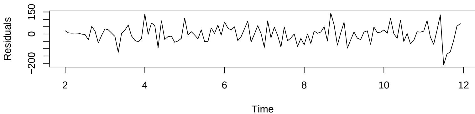
Interpolation Prediction Errors
