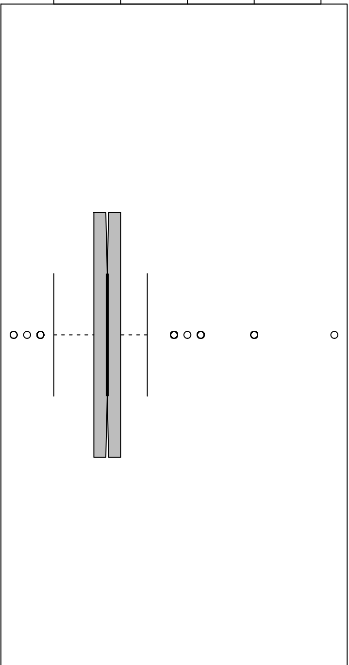
Boxplot Tomorrowland
