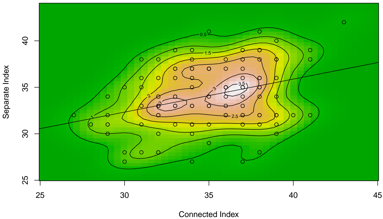
Bivariate Kernel Density – Y2010
