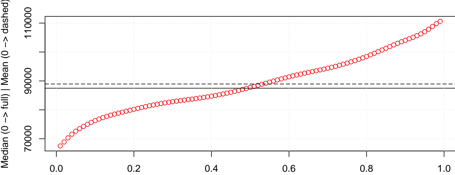
Harrell-Davis Quantiles
