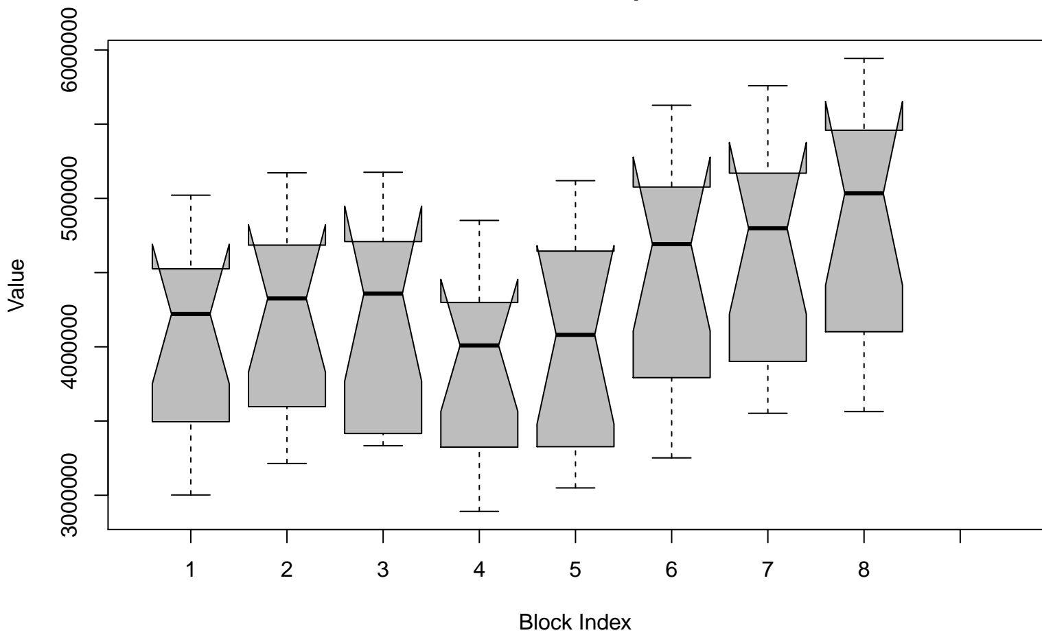
Notched Box Plots – Sequential Blocks
