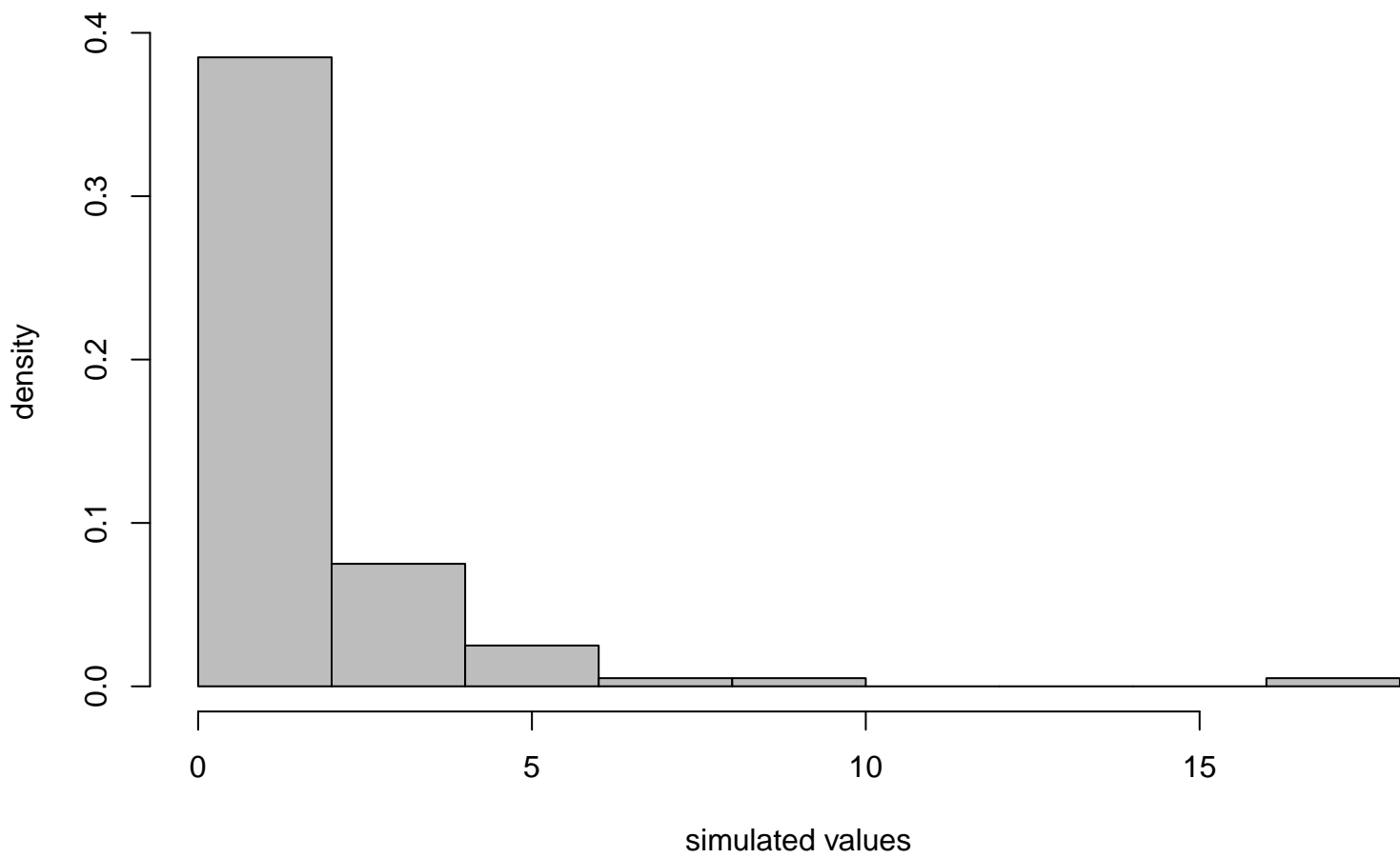
Histogram of 1st simulated series
