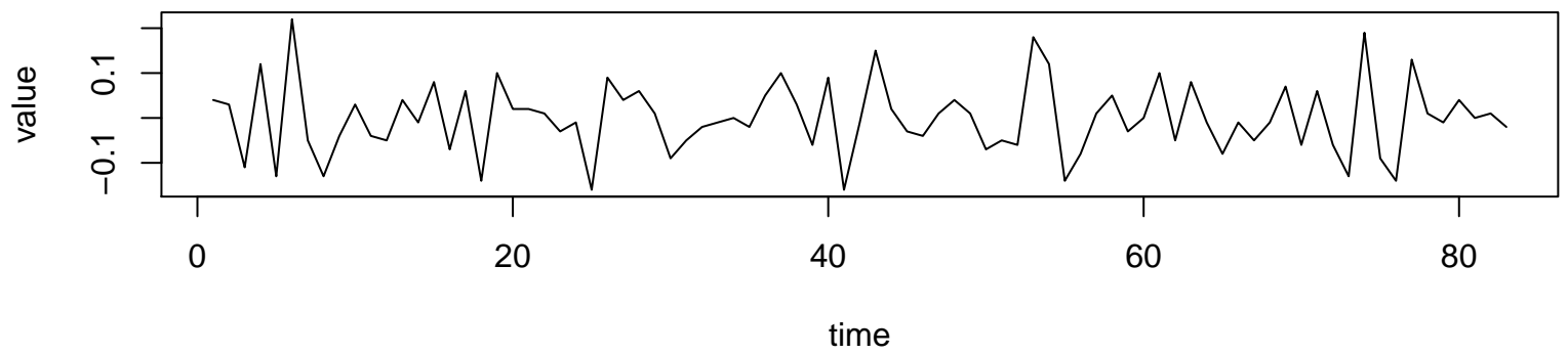
Working Time Series ( \lambda=1, d=1, D=1 )
