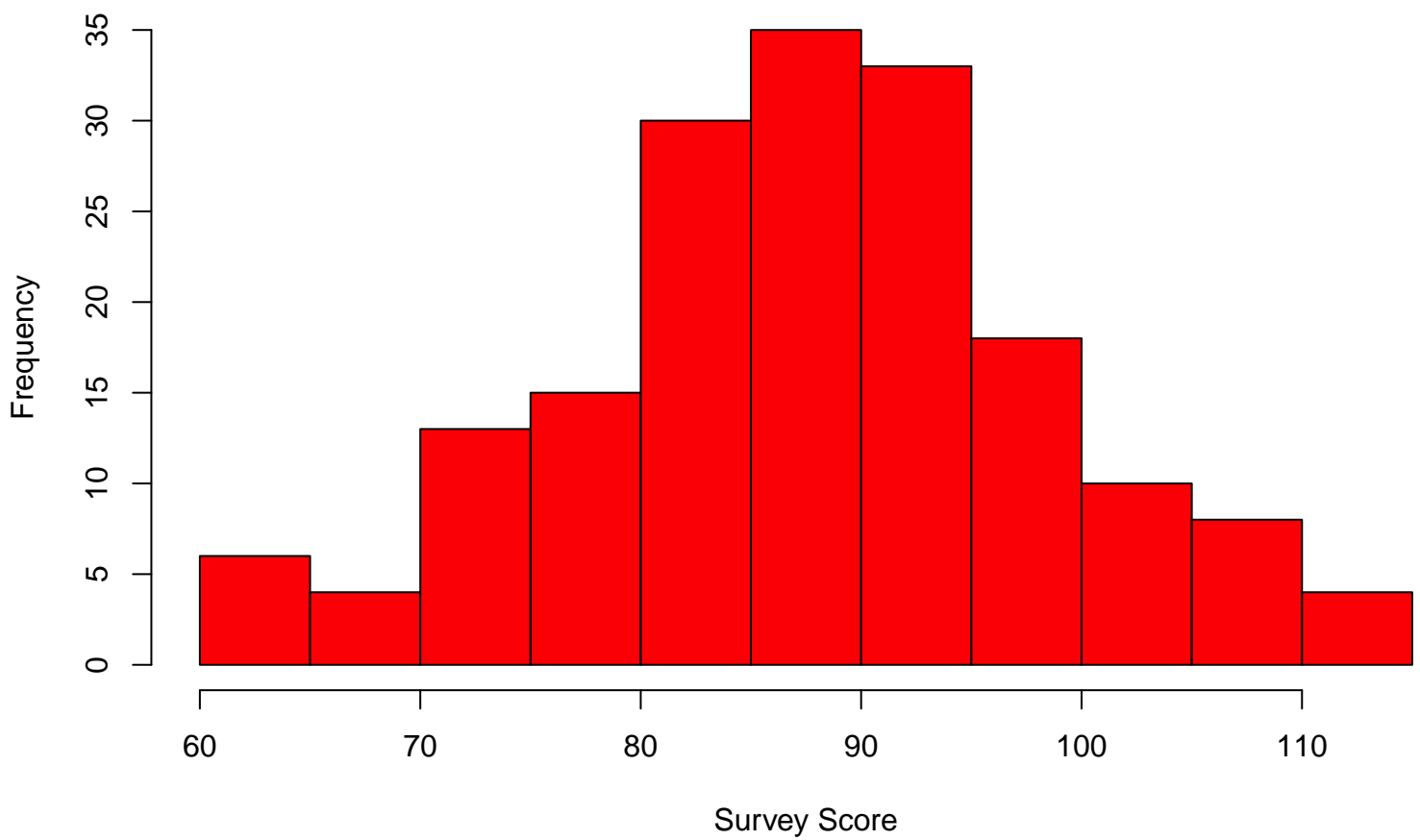
Histogram of WS1 data
