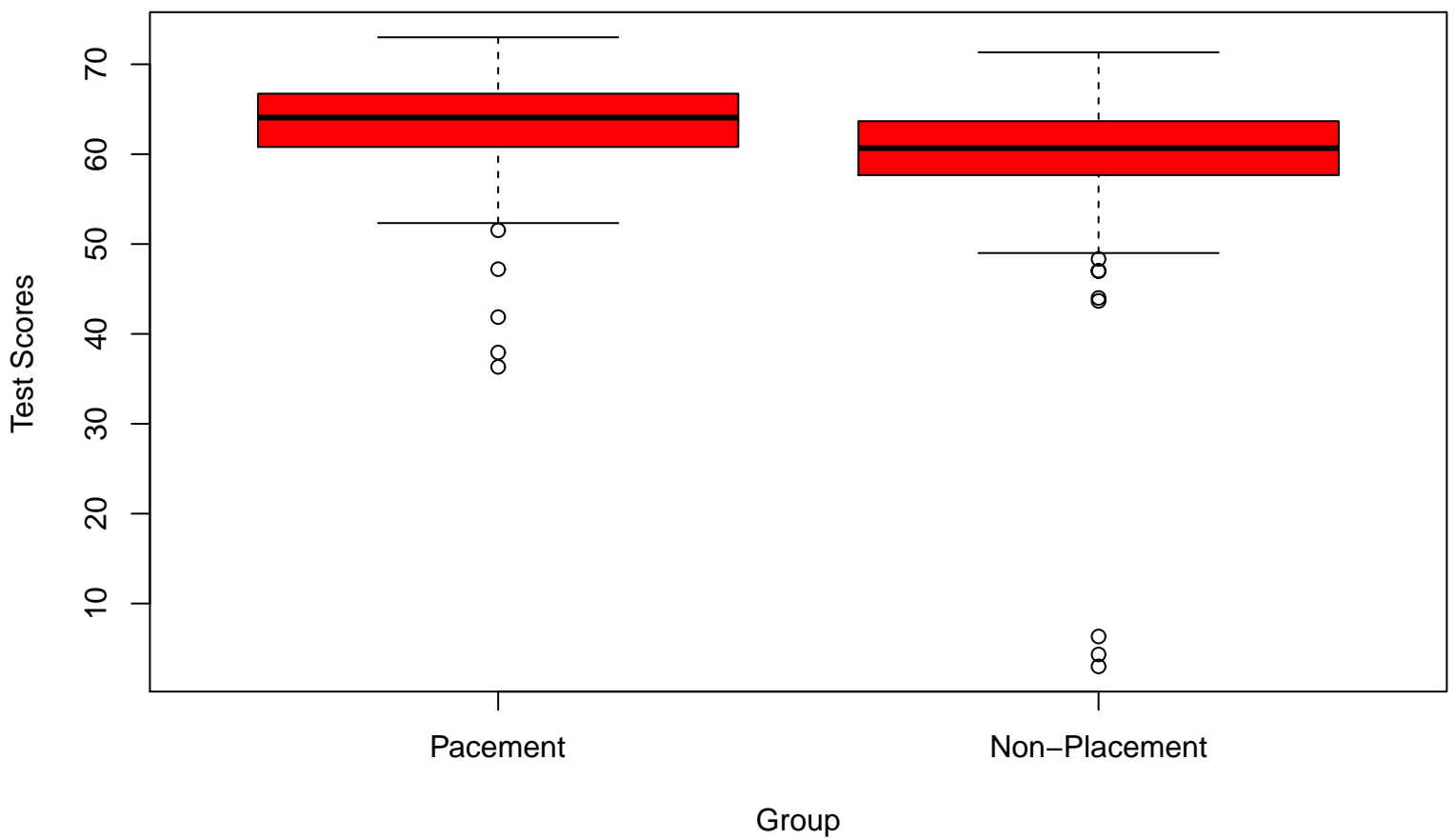
Difference in scores between P and NP
