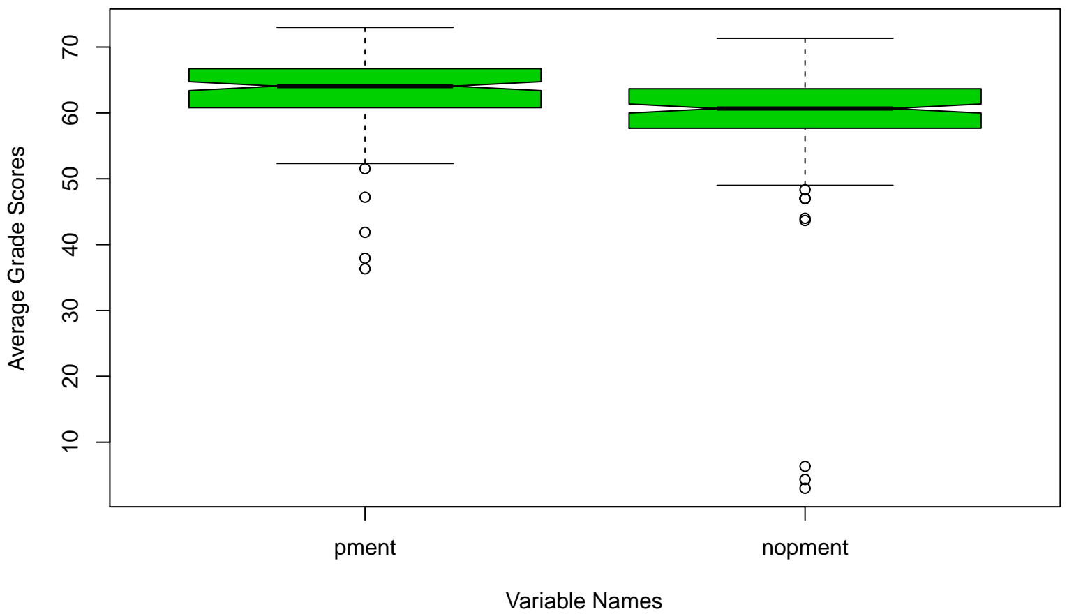
Effect of doing a placement on grades
