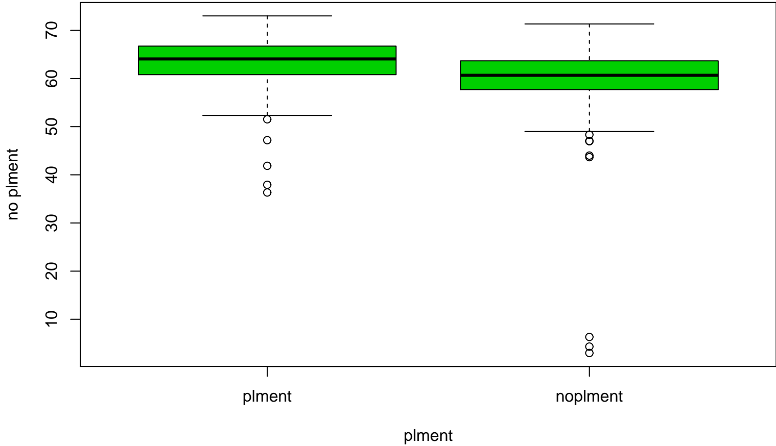
No/Placement Scatterplot
