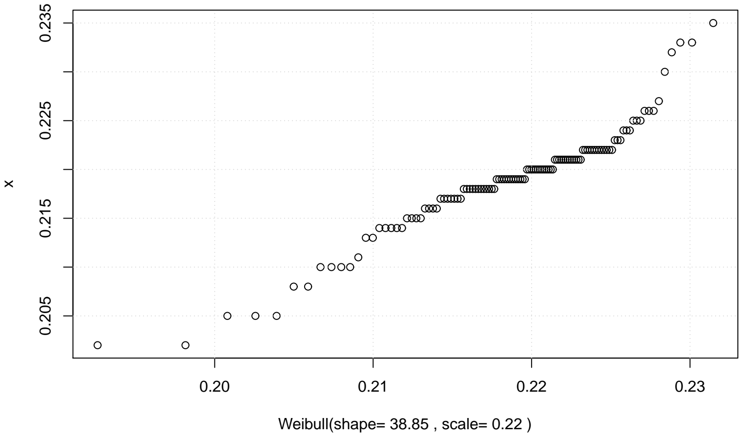
QQ plot (Weibull)
