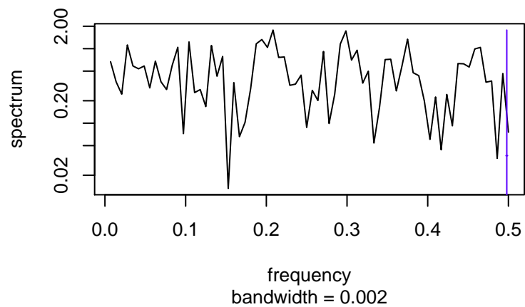
Standardized Residuals
