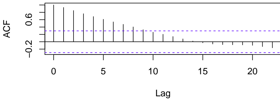
ACF of x (raw)
