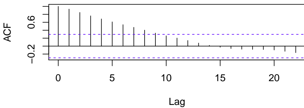
ACF of x (transformed and differenced)
