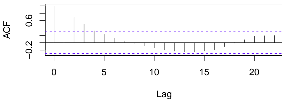
ACF of y (transformed and differenced)
