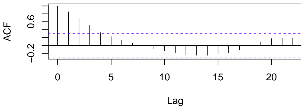
ACF of y (raw)
