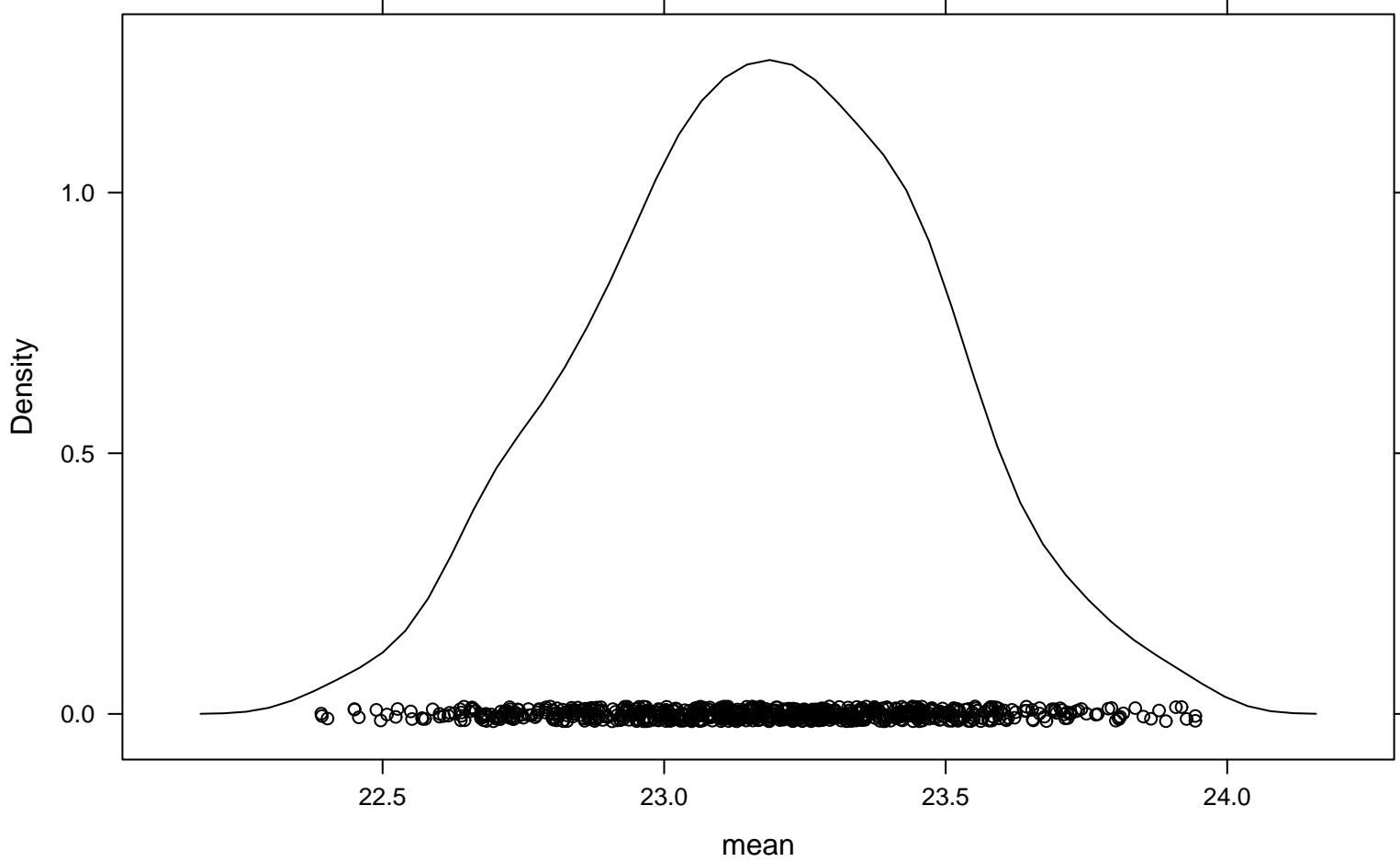
Density Plot
